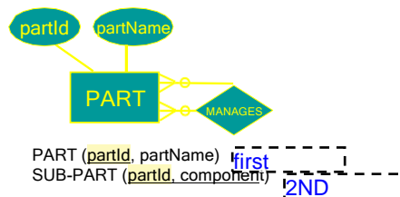
Fig. 4: Recursive many to many relationship and transformation
