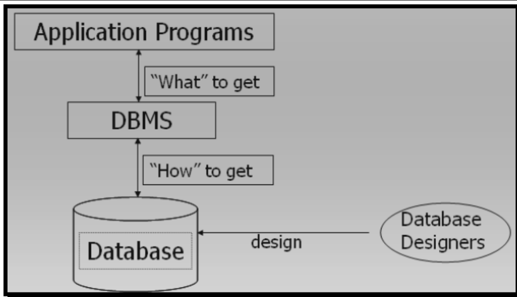
Fig. 5: Database Designers
