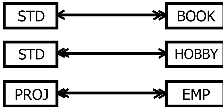
Fig. 2: Arrow-head notation
