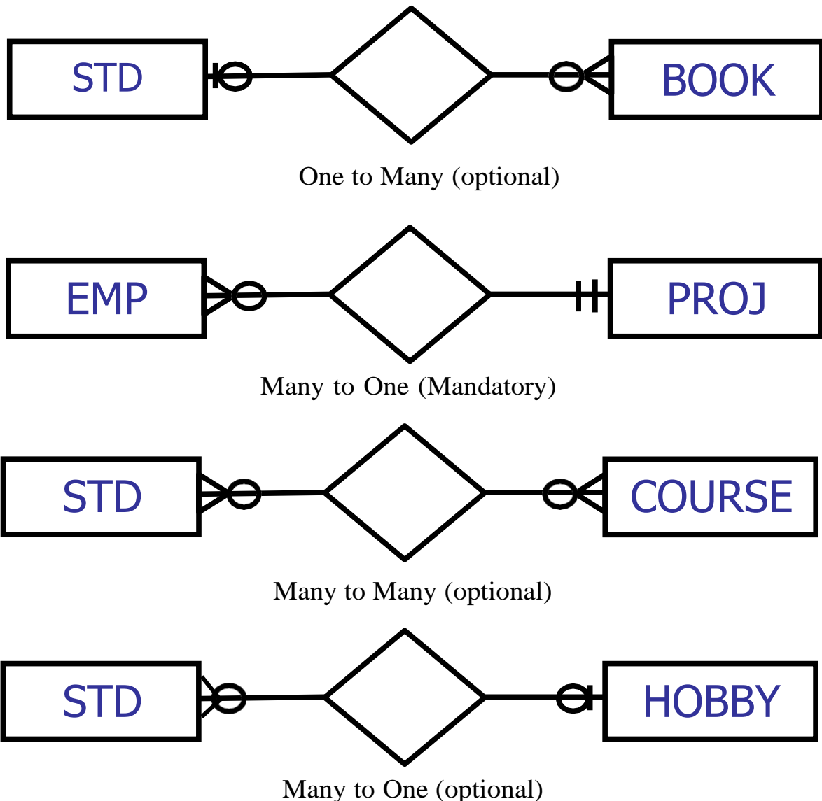
Fig 1: Different Cardinalities
